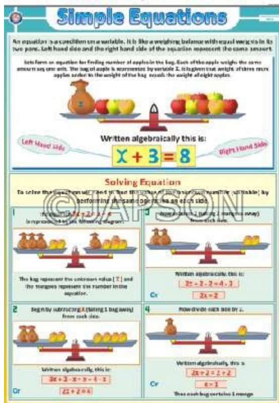
I. Charts, Simple Equations
