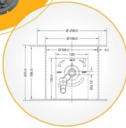
8" Duct Damper
