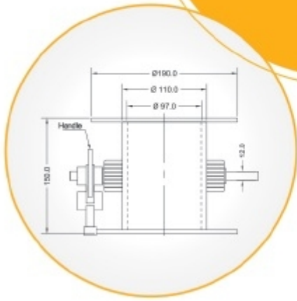
4" Duct Damper
