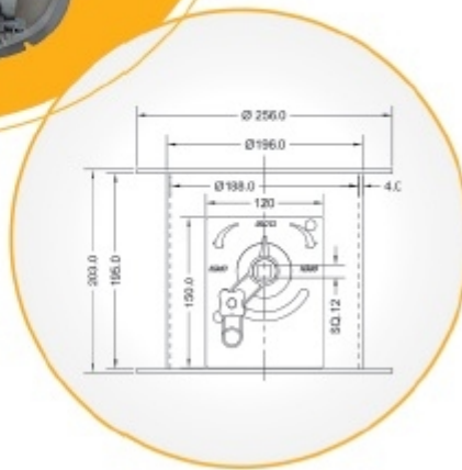
8" Duct Damper
