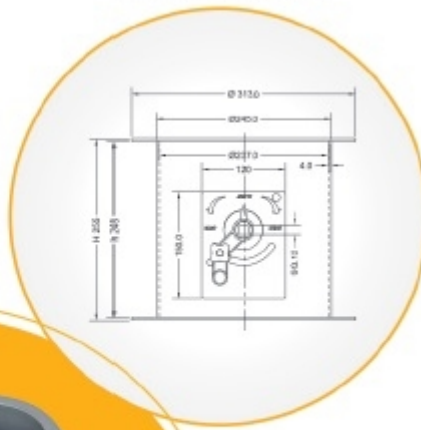
10" Duct Damper
